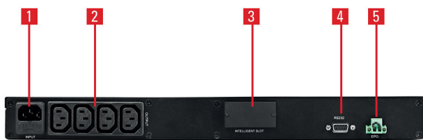
SPS 750 ÷ 1500 ADV R
